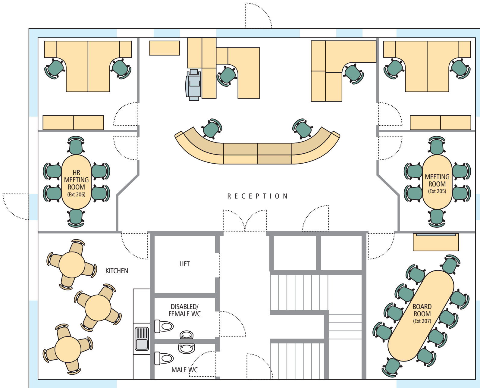
Teal House – Ground Floor Layout
